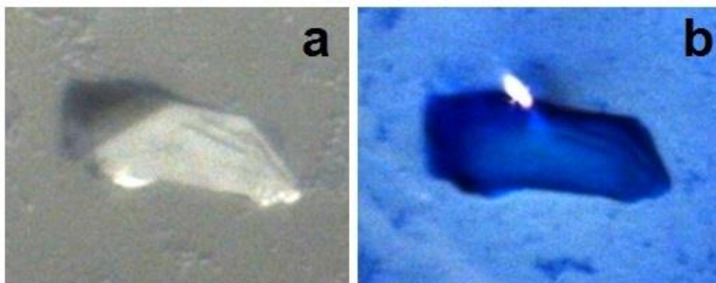
Figure 1. Protein crystal; a) observed in B4-well of Salt Rx screen at 18°C on 28 th day of incubation with 1.8 M ammonium citrate dibasic and 0.1 M sodium acetate trihydrate at pH 4.6, b) after staining with IZIT dye solution on 40 th day of incubation.
